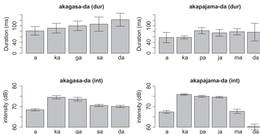
Figure 8: Duration and intensity of each vowel in the sentences shown in Figure 5. The data come from the acoustic analysis of Kawahara et al. (2015).
