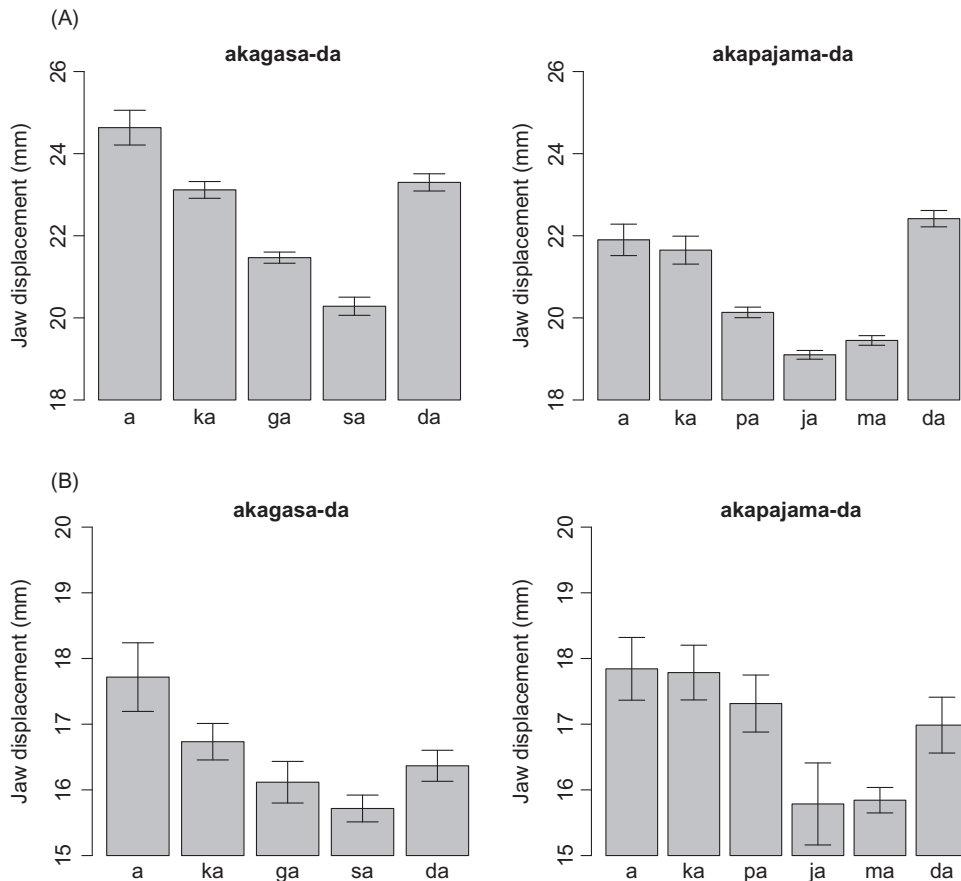
Figure 5: Jaw displacement patterns of Japanese sentences consisting of syllables with [a] (two speakers). Taken from Kawahara et al. (2014). Reprinted with permission.
