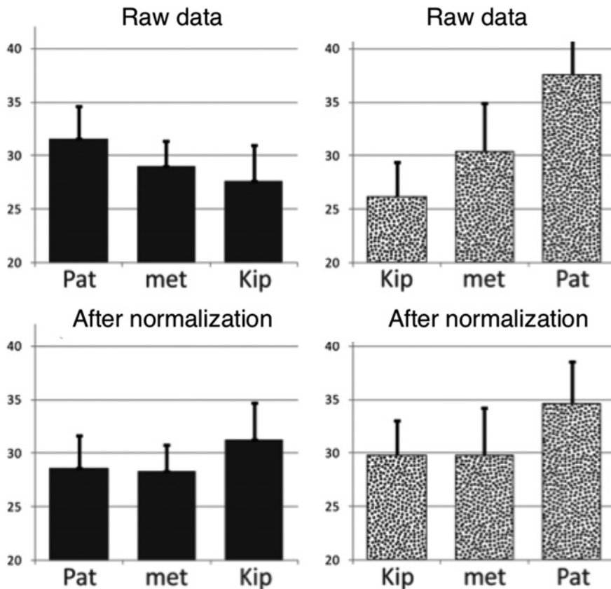
Figure 4: Top panel shows the raw jaw movement of “Pat met Kip” (left) and “Kip met Pat” (right), and bottom panel shows the normalized data for the two sentences. Sentential stress is on the last word. Taken from Erickson et al. (2014c).
