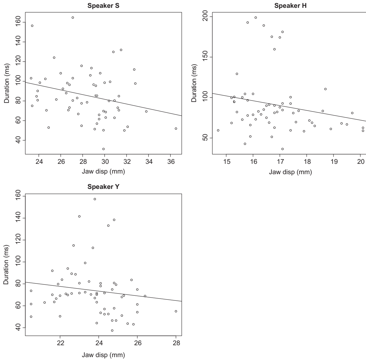
Figure 7: Correlation between duration and jaw displacement in Japanese.
