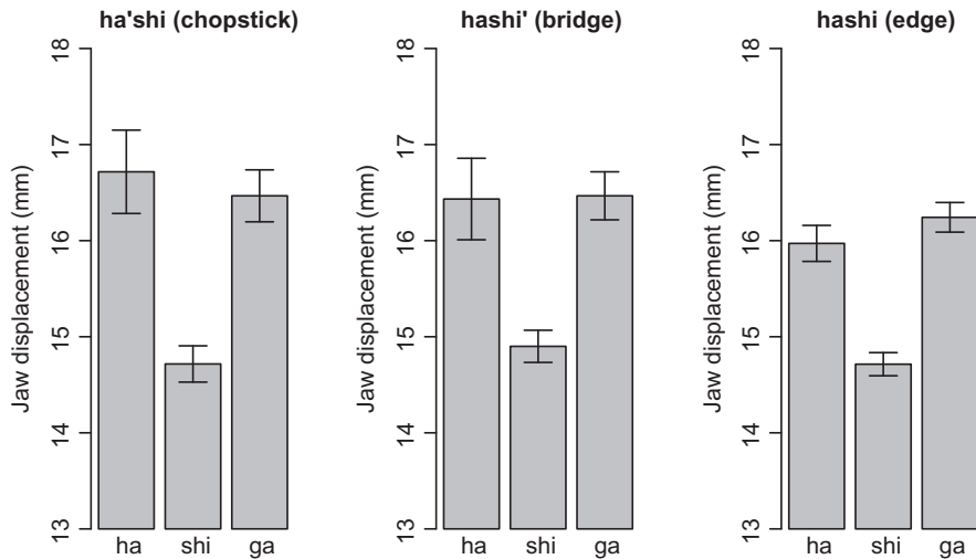
Figure 6: Jaw displacement patterns of Japanese triplets that differ in accentual placement. Taken from Kawahara et al. (2014). Reprinted with permission.
